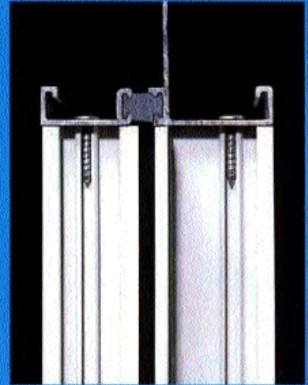
Cross section reveals coping and thermal break construction.
