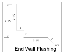
End Wall Flashing
