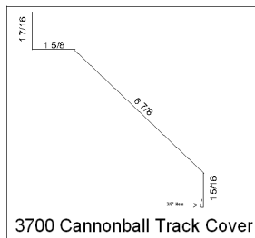
3700 Cannonball Track Cover
