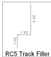
RC5 Track Filler
