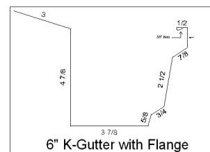
6" K-Gutter with Flange
