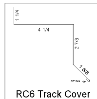
RC6 Track Cover
