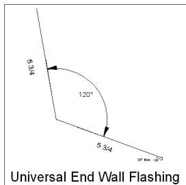
Universal End Wall Flashing
