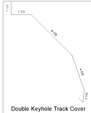
Double Keyhole Track Cover
