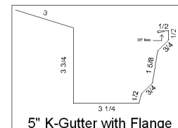
5" K-Gutter with Flange
